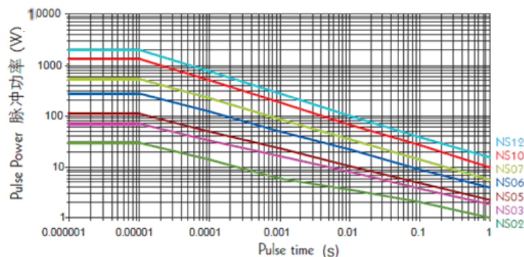
NS02, NS03, NS05, NS06, NS07, NS10, NS12 one-pulse limiting power
