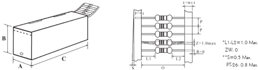
Dimension of T/B (mm)
