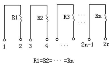
B TYPE(Isolated):
