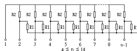
RTYPE(Dual Terminator)
