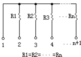
A TYPE(Bussed)
