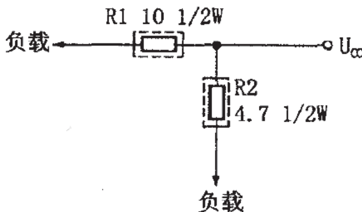
(Fig.3: Application circuit of fusing resistors)
